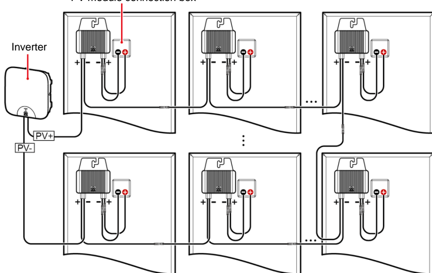
PV module connection box
